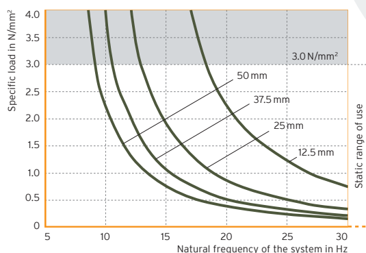
Fig. 3: Natural frequencies for different bearing thicknesses
