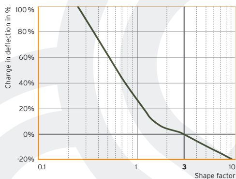
Fig. 7: Deflection³ in relation to the shape factor
