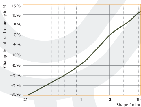
Fig. 9: Natural frequency³ in relation to the shape factor
