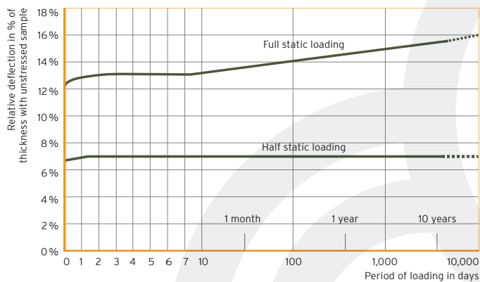
Fig. 4: Deformation under static load depending on time
