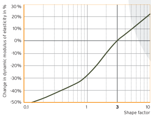
Fig. 8: Dynamic modulus of elasticity³ at 10 Hz in relation to the shape factor
