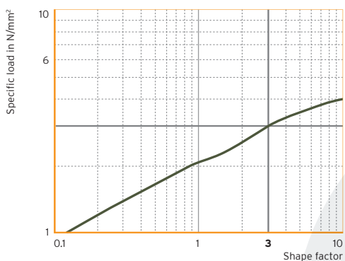
Fig. 6: Static range of use in relation to the shape factor
